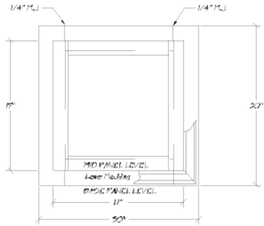
COLUMN CUTAWAY BELOW UPPER MOULDING
