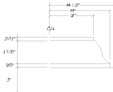
COLUMN BASE DETAIL
