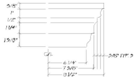
COLUMN CAP DETAIL
