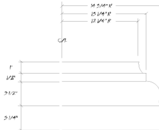
Base Detail
