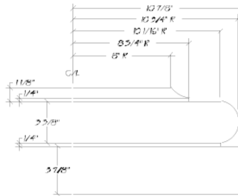
Base Detail
