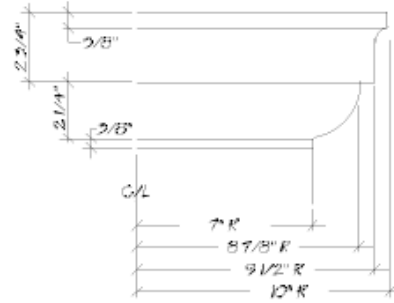
Cap Detail
