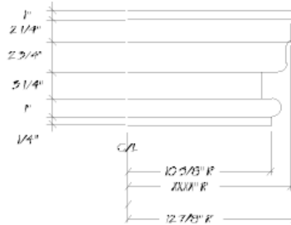
Cap Detail
